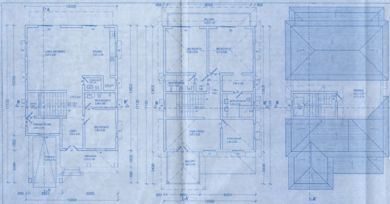
TYPICAL GROUND FLOOR PLAN FOR BLOCK 'A1', BLOCK 'A2', BLOCK 'A3', BLOCK 'A4' AND BLOCK 'A5' SCALE - 1:100
