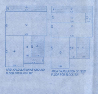
AREA CALCULATION OF GROUND FLOOR FOR BLOCK 'B2' SCALE - 1:100
