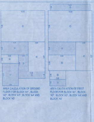
AREA CALCULATION OF GROUND FLOOR FOR BLOCK 'A1', BLOCK 'A2', BLOCK 'A3', BLOCK 'A4' AND BLOCK 'A5' SCALE - 1:100
