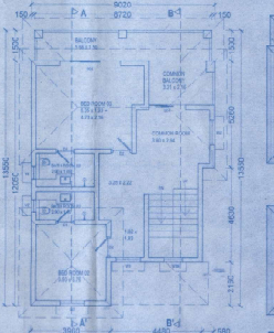
FIRST FLOOR PLAN FOR BLOCK 'B2' SCALE - 1:100
