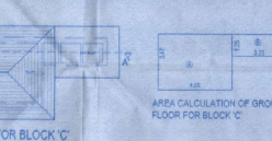
ROOF PLAN FOR BLOCK 'C' SCALE - 1:100
