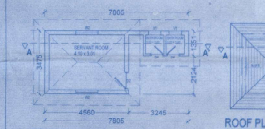
GROUND FLOOR PLAN FOR BLOCK 'C' SCALE - 1:100
