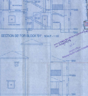
SECTION B-B' FOR BLOCK 'B1' SCALE - 1:100
