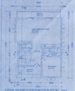
TYPICAL GROUND FLOOR PLAN FOR BLOCK 'B1' SCALE - 1:100
