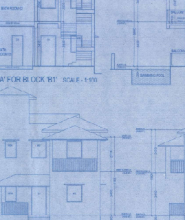
SECTION B-B' FOR BLOCK 'B2' SCALE - 1:100
