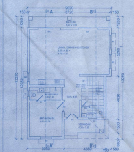
GROUND FLOOR PLAN FOR BLOCK 'B2' SCALE - 1:100
